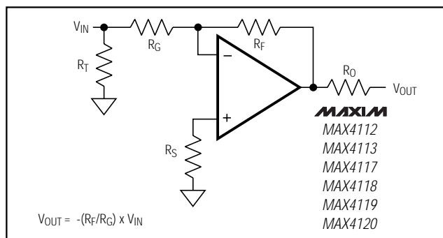
Figure 2a. Inverting Gain Configuration
